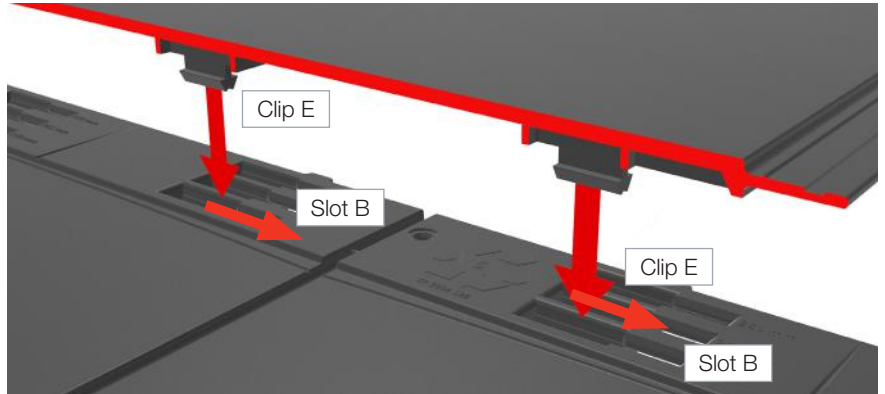
Envirotiles are clipped together using the two clips on the underside at the bottom of the tile (E) clipping into the slots at the top of the tile on the course below (B). Note that the tile must be aligned, then pushed down, then the tile is slid to the right to lock into the clip. The sliding action also locks the connecting strip into the adjacent tile slot.
