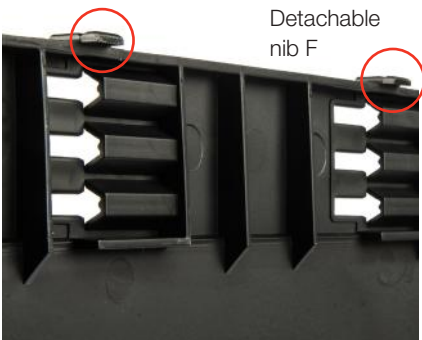
Each tile has two detachable nibs (F) at the top. These are used to hook the tile over the batten. When a batten has been fitted out of alignment or there has been some movement after fitting, the installer can break the nibs off as required if they find that the nibs no longer hook over the batten.
